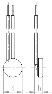
Diameter d 9,0 mm Installation height h ab 3,9 mm
